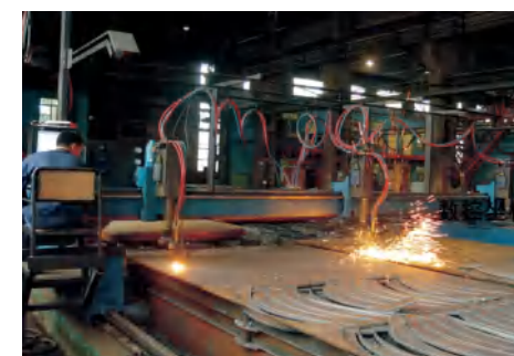
↑ 数控坐标式火焰切割机 Japanese Automatic Flame Cutting machine
